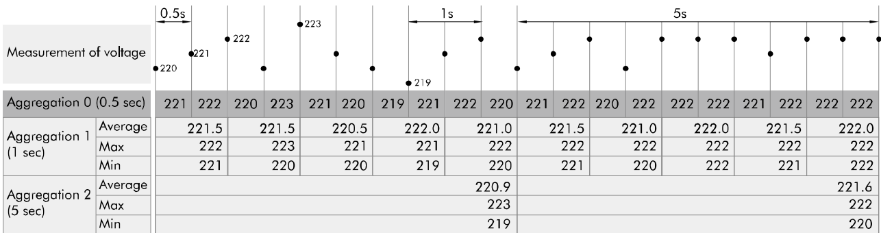
Fig 2.7 Aggregation of measured data
